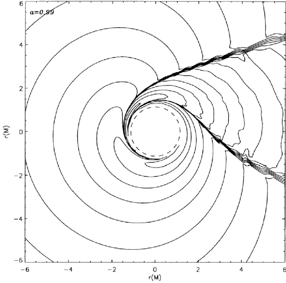
Figure 5.2: General relativistic hydrodynamics simulation on the Kerr geometry. Iso-contours of the logarithm of the matter density are shown for extreme Kerr, a = 0.99 M . A shock is wrapped around the Kerr black hole. The outer boundary is placed at 50.9 M , and the inner boundary is identical with the outer horizon at 1.14 M . The adiabatic index of the perfect fluid is \gamma = 5/3 , asymptotic Mach number amounts to 5.0. (Credit: [Fon99])
