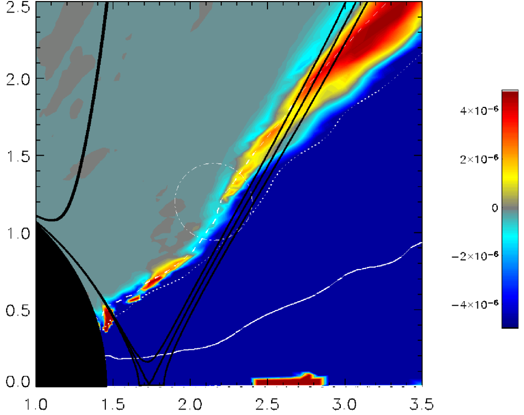
Figure 5.9: Color-coded radial azimuthally-averaged mass flux, \langle \rho U^r \rangle_\phi , as a result of the decay of an initial torus configuration simulated with non-radiative 3D GRMHD. The main disk body is displayed by white contour lines: 10^{-1} \rho_{\max} ( solid ), 10^{-2} \rho_{\max} ( dotted ), 10^{-3} \rho_{\max} ( dashed ). Below 10^{-3} \rho_{\max} the tenuous axial funnel is illustrated in gray color. The circle indicates the base of the jet where outgoing and ingoing material can be found. The thick black lines mark equipotential surfaces for marginally bound gas to display unbound outflows, \Phi_{\text{mb}} = [-0.01, 0, 0.01] . Parameters were also chosen to the KDP model as in Fig. 5.8 (Credit: [DeV04]).
