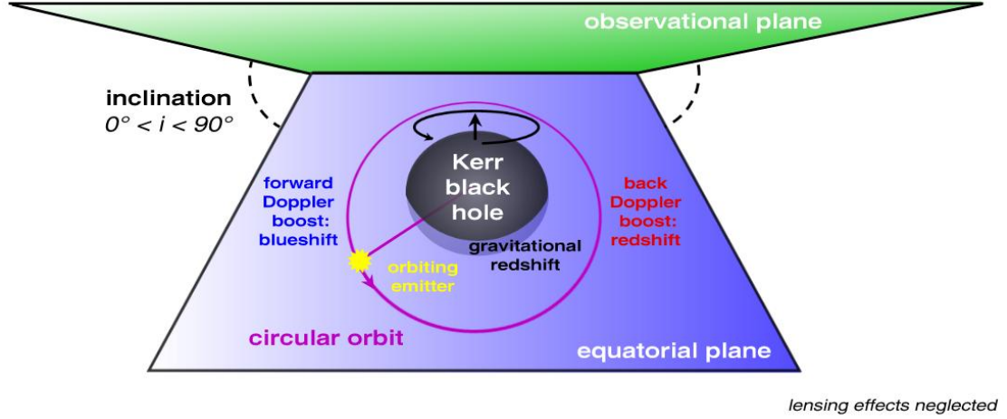
Figure 3.5: Illustration of an emitter circulating a black hole on a circular Keplerian orbit. The observer is assumed to look at intermediate inclination onto the orbital plane. The nearness to the black hole’s horizon causes relativistic modulations of the intrinsic emission spectrum: Beaming and back beaming provoke periodical flickering of the orbiting source. Gravitational redshift dims the emission. The time-dependence of an intrinsic light curve is disturbed by time dilation effects. All these effects are contained in the generalized fully relativistic Doppler factor ( g -factor).
