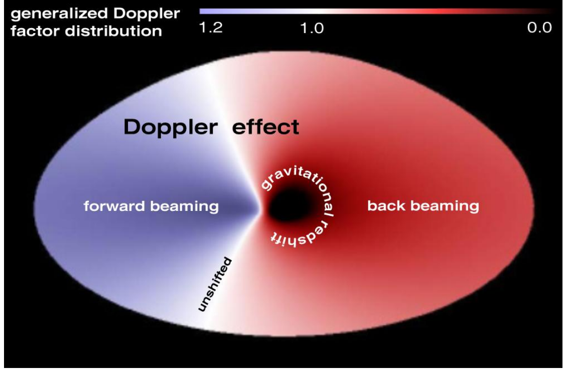
Figure 6.2: Simulated disk image around a central Kerr black hole color-coded in the generalized Doppler factor g . The distribution illustrates redshift g < 1 ( black to red ), no shift g = 1 ( white ) and blueshift g > 1 ( blue ). Regions of Doppler effect, beaming and gravitational redshift are marked. The inclination angle amounts i = 60^\circ .
