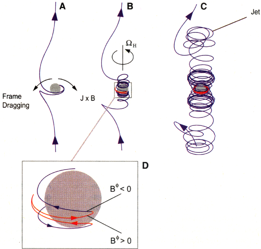
Figure 5.7: Evolving structures of a single magnetic flux tube embedded in a magnetosphere in the Kerr geometry. The frame-dragging effect wraps the initial flux tube (a) around the black hole spin axis. Then, the black hole ergosphere drives a Poynting flux (b). The result of this dynamics is a bipolar structure (c), a "magnetic tower": a jet . The red portions indicates plasma with negative total energy as viewed from infinity (compare Penrose process in Sec. 3.5). The gravitomagnetic dynamo is shown in the small close-up (d). Here, the azimuthal component of the magnetic field changes sign. The Alfvén speed amounts 12c to 13c in the regions where the ergospheric Poynting flux drives the jet. (Credit: [Sem04a])
